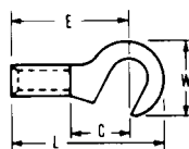
Basic Dimensions
